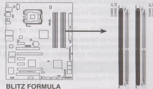
BLITZ FORMULA 240-pin DDR2 DIMM sockets
