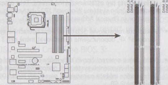
MAXIMUS FORMULA(Special Edition)/ MAXIMUS FORMULA 240-pin DDR2 DIMM sockets
