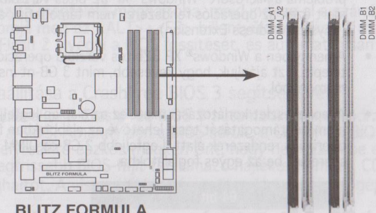
BLITZ FORMULA 240-pin DDR2 DIMM sockets
