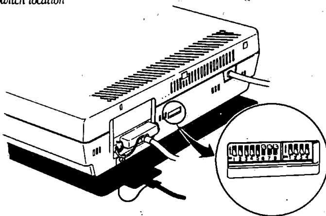
Figure D-1. DIP switch location
