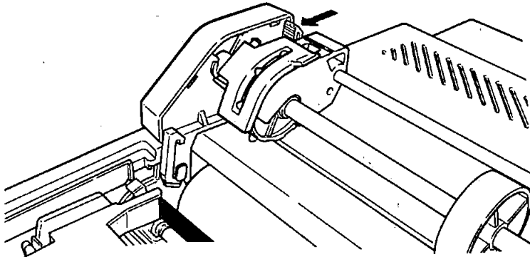
Figure 1-10. Locking lever for pin feed holder adjustment
