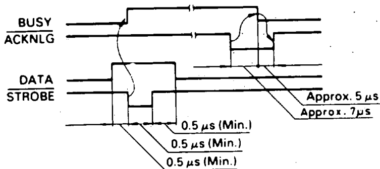
Figure F-1. Parallel interface timing
