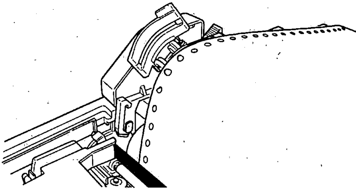
Figure 1-12: Fitting the paper into the left pin feed holder
