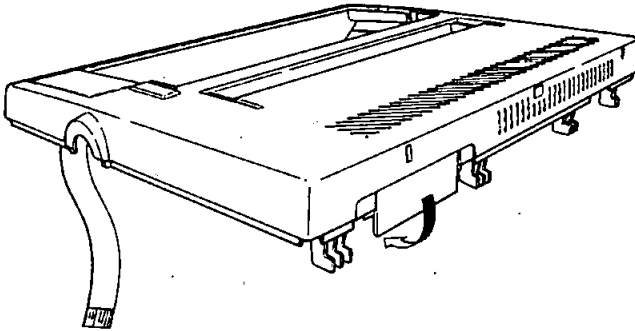
Figure E-3. Connector cover
