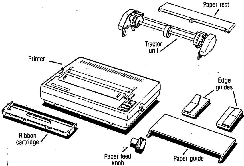
Figure 1-1: Printer parts
