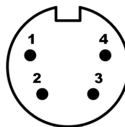
DIN-4 plug, view on the pins
