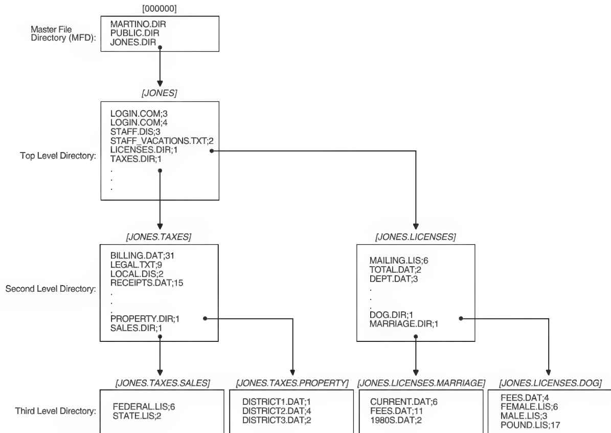
Figure 4–1 Directory Structure
