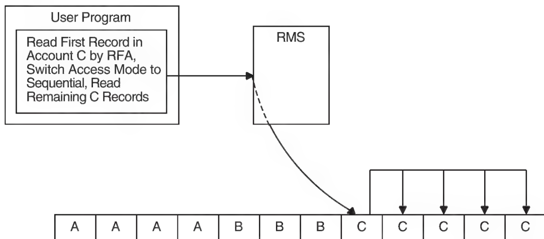
Figure 8–1 Using RFA Access to Establish Record Position
