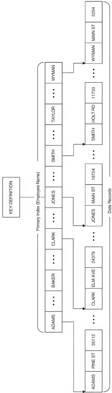
Figure 2-12 Single-Key Indexed File Organization
