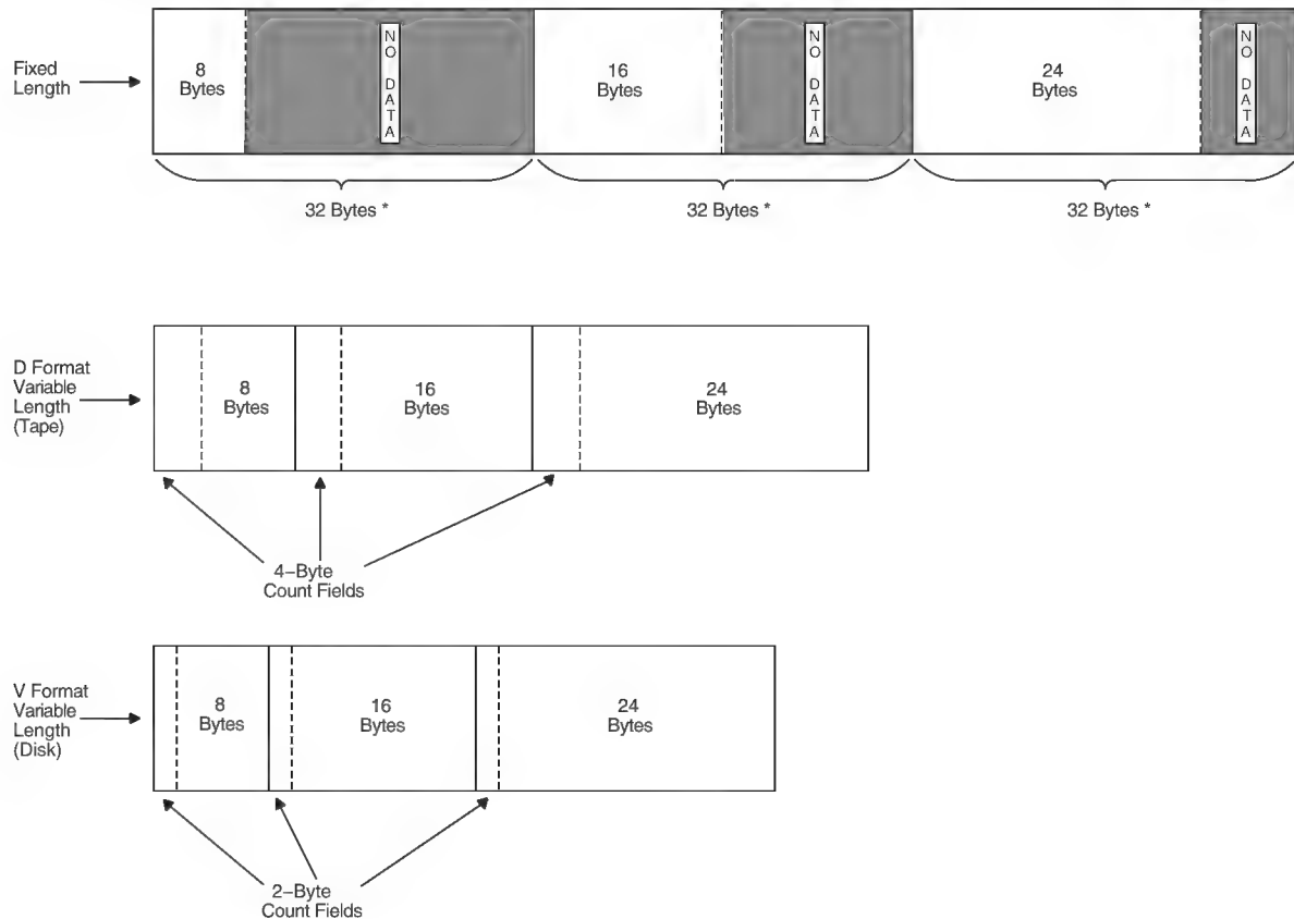
Figure 2-6 Comparison of Fixed- and Variable-Length Records
