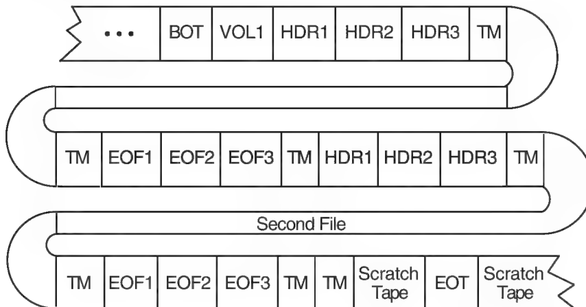
Figure 1–9 Multifile/Single-Volume Configuration
