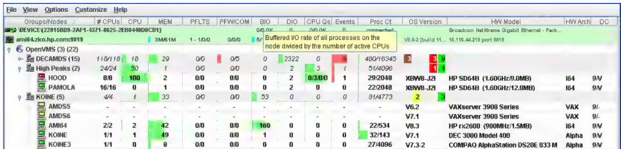
Figure 3–2 Sample Tooltip
