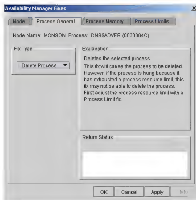
Figure 6–4 Delete Process
