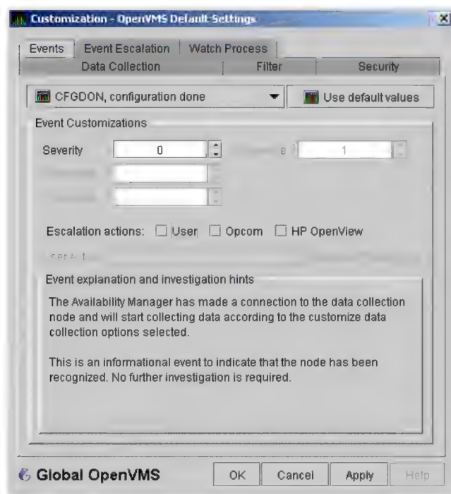
Figure 7–19 Event Customizations
