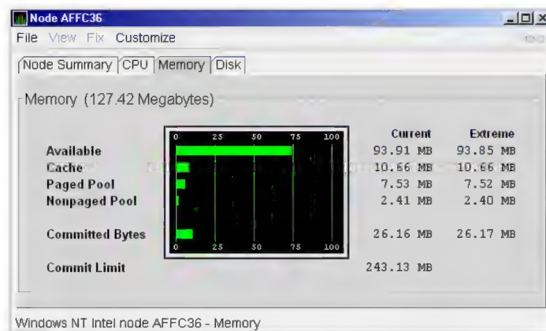
Figure 3–9 Windows Memory
