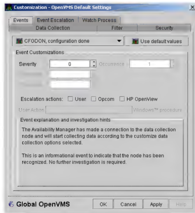
Figure 7–18 Event Customizations
