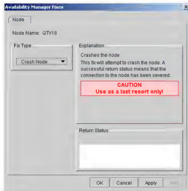
Figure 6–2 Crash Node
