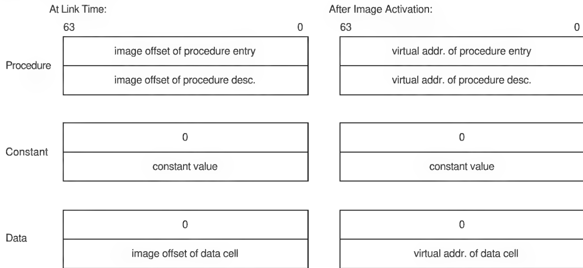
Figure 6-1 Symbol Vector Contents
