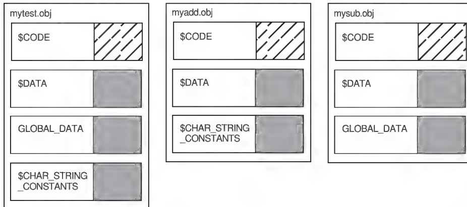
Figure 7–2 Program Sections Created for Examples 3-1, 3-2, and 3-3
