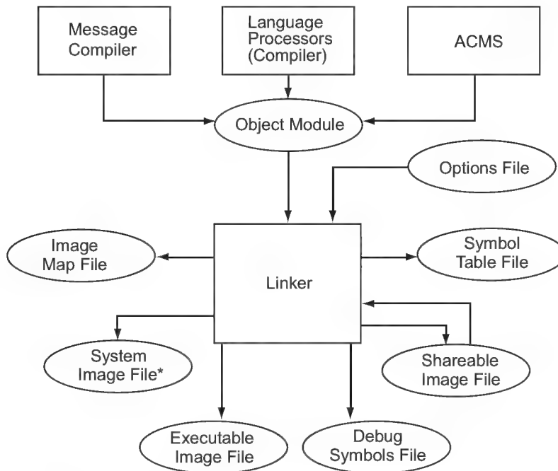
Figure 1–1 Position of the Linker in Program Development
