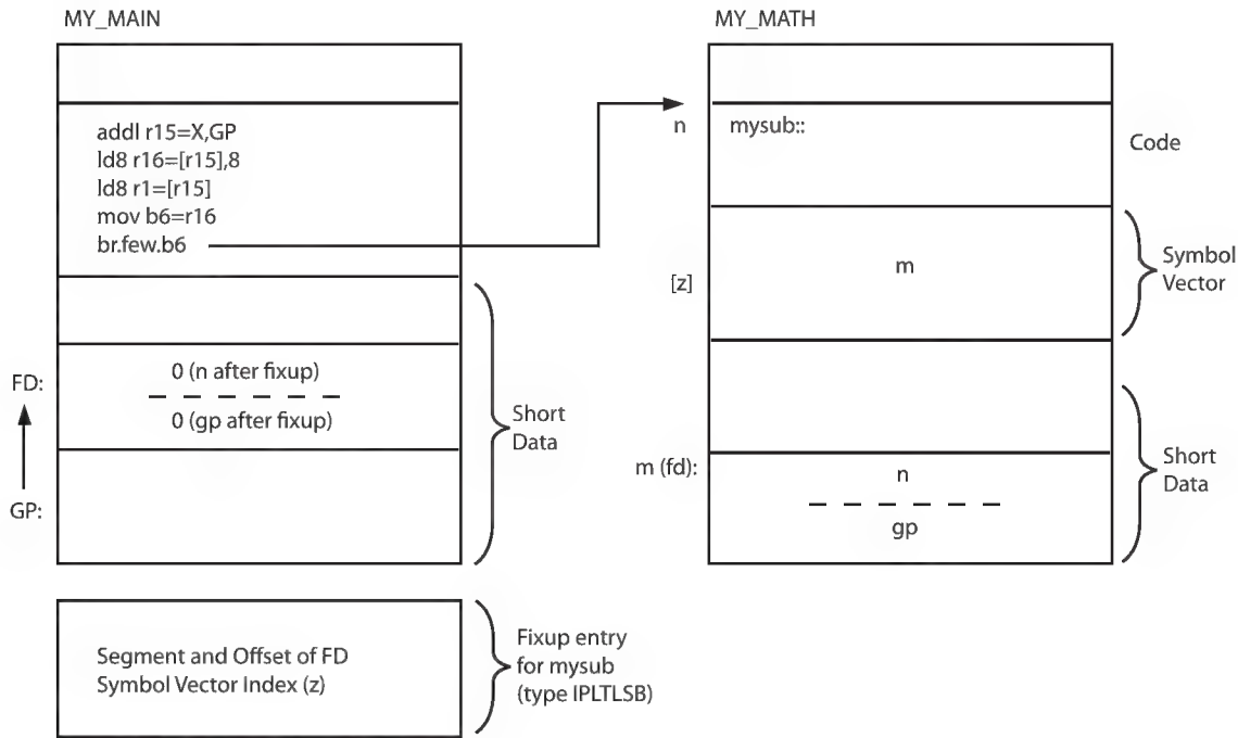
Figure 4–1 Accessing Universal Symbols Specified Using the SYMBOL_VECTOR= Option
