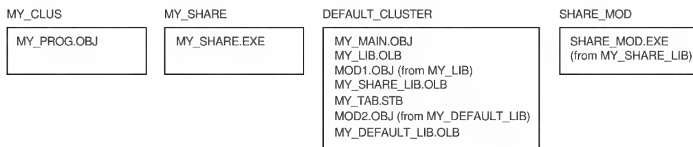
Figure 6–3 Clusters Created for Sample Link
