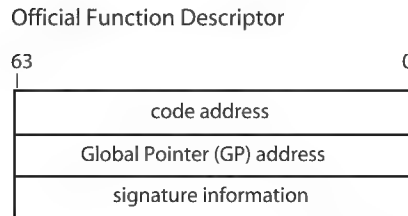
Figure 3–3 Official Function Descriptor
