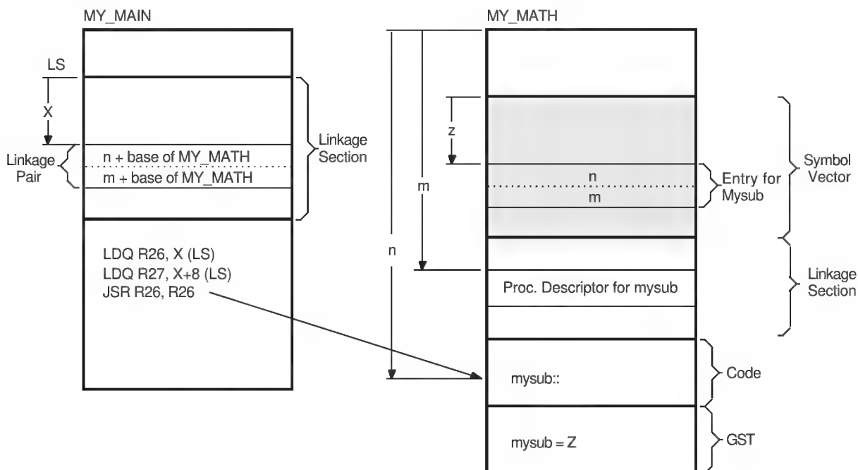
Figure 8-2 Accessing Universal Symbols Specified Using the SYMBOL_VECTOR= Option
