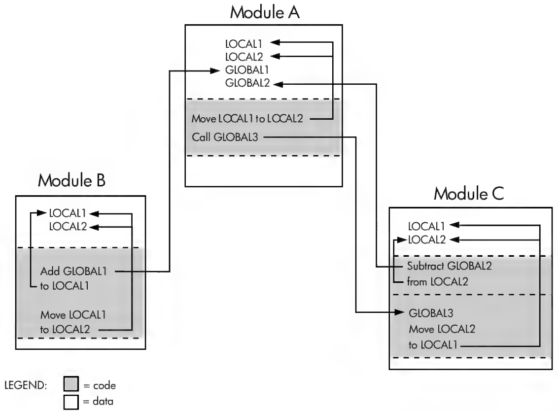
Figure 2-2 Symbol Resolution
