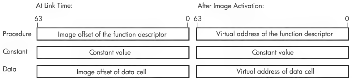
Figure 2–1 Symbol Vector Contents
