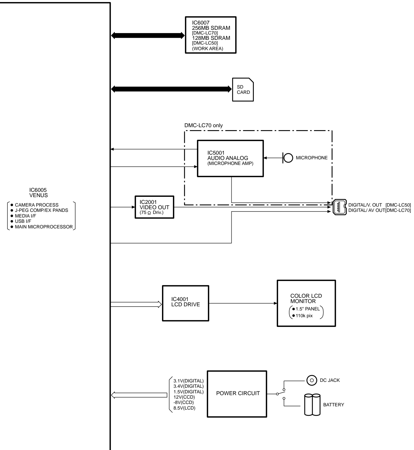
DMC-LC50/LC70PP/PL/EB/EG/EGM/GC/GD/GN OVERALL BLOCK DIAGRAM
