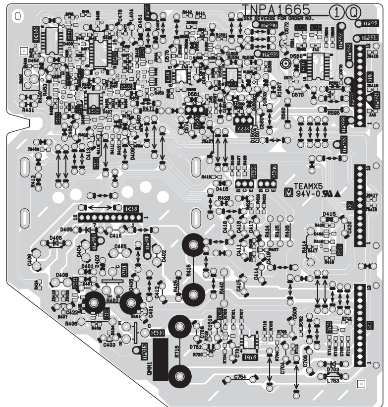
Q-Board Layout
