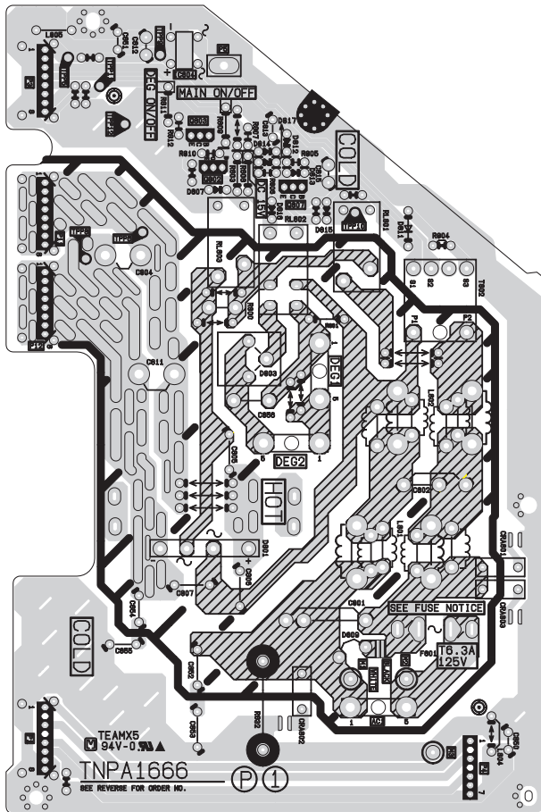
P-Board Layout
