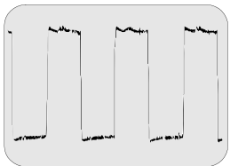
41 Q-Board Q10 Pin 4 - 4.16V p-p H-DRIVE
