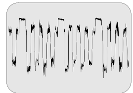
45 L-Board IC3803 Pin 8 - 166.00V p-p B-DRIVE
