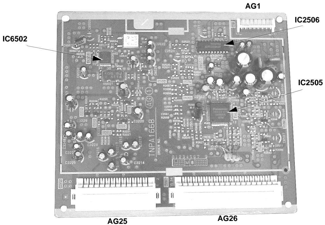
Figure 54. AG-Board
