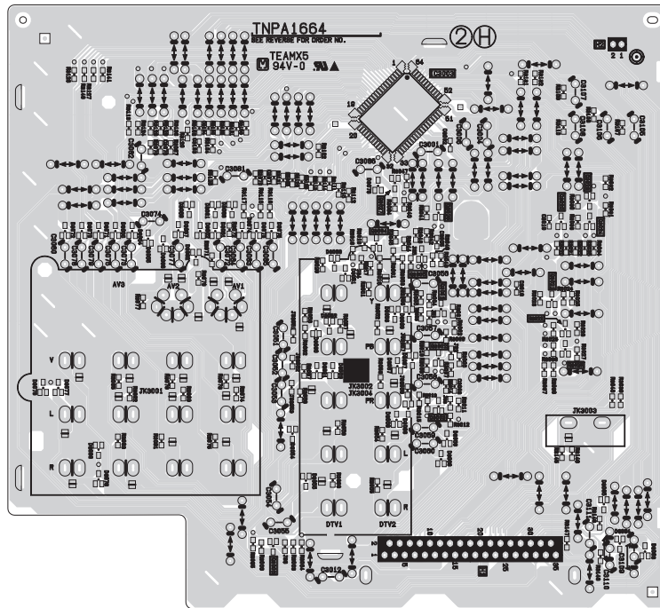
H-Board Layout
