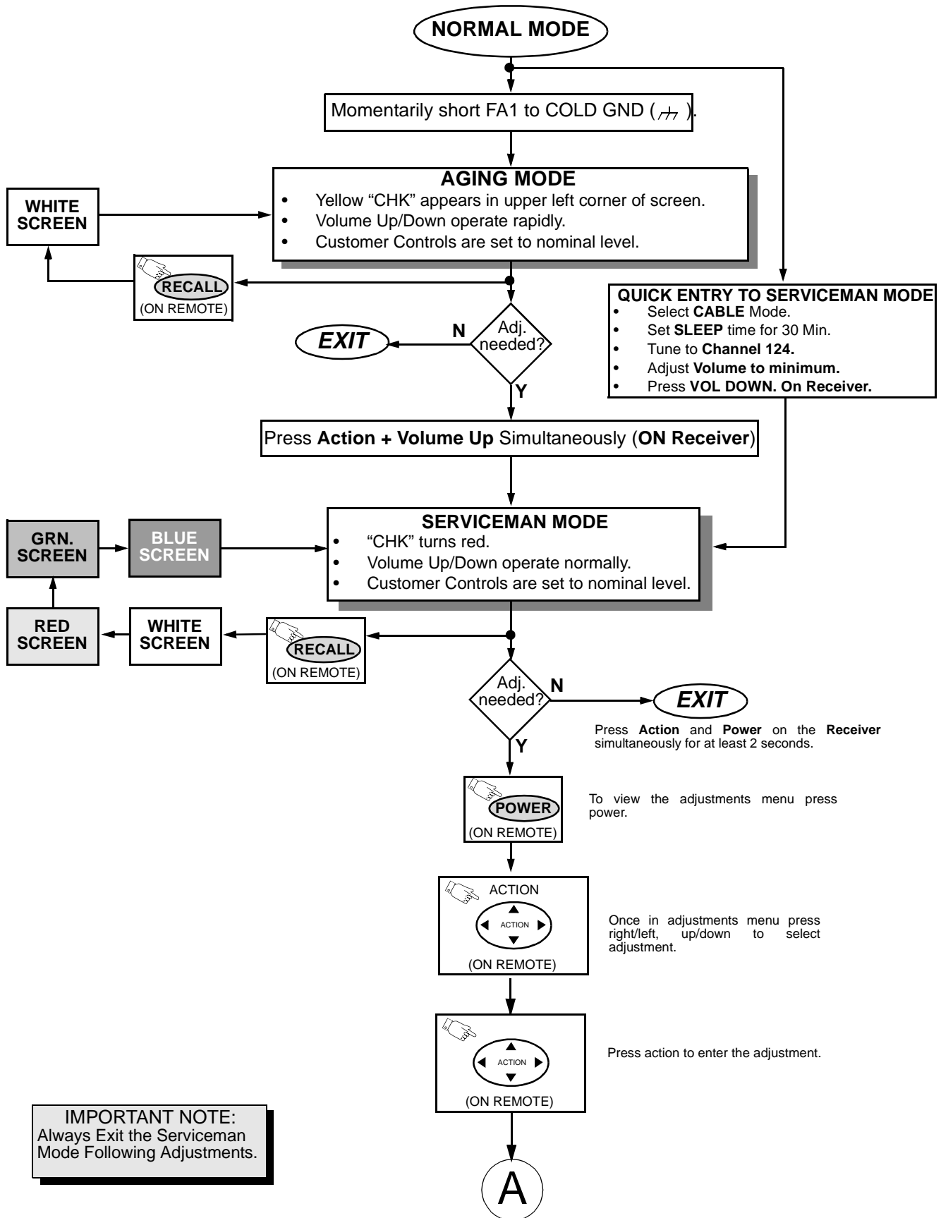
Figure 22. Flow Chart for Serviceman Mode.
