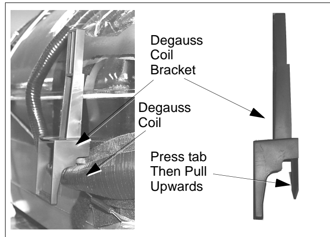
Figure 7. Brackets removal
