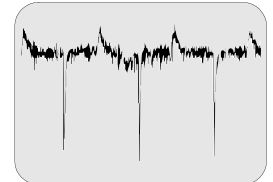
⑮ A-Board IC001 Pin 4 - 0.33V p-p VERSION
