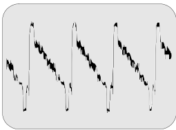
①⑥ A-Bboard IC001 Pin 28 - 1.86V p-p CVBS0
