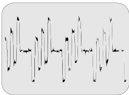
②⑥ A-Bboard A26 Pin 12 - 1.53V p-p SUB V/Pb
