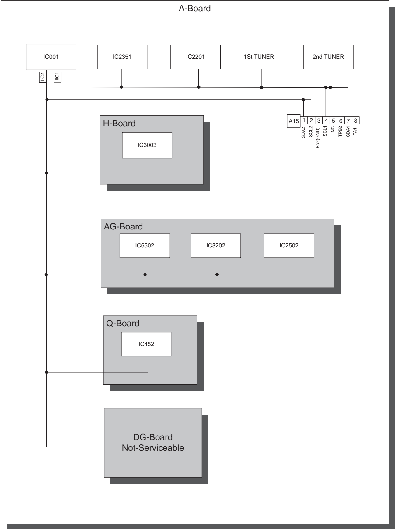
Figure 47. IIC Connection
