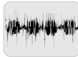
①⑨ A-Bboard A25 Pin 9 - 0.24V p-p S/VIDEO SW
