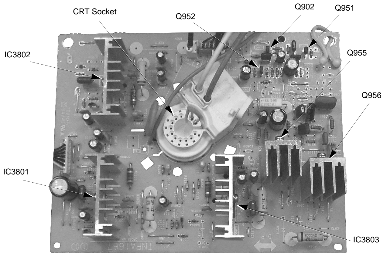
Figure 52. L-Board
