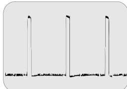
② A-Board IC001 Pin 49 - 3.56V p-p H-SYNC
