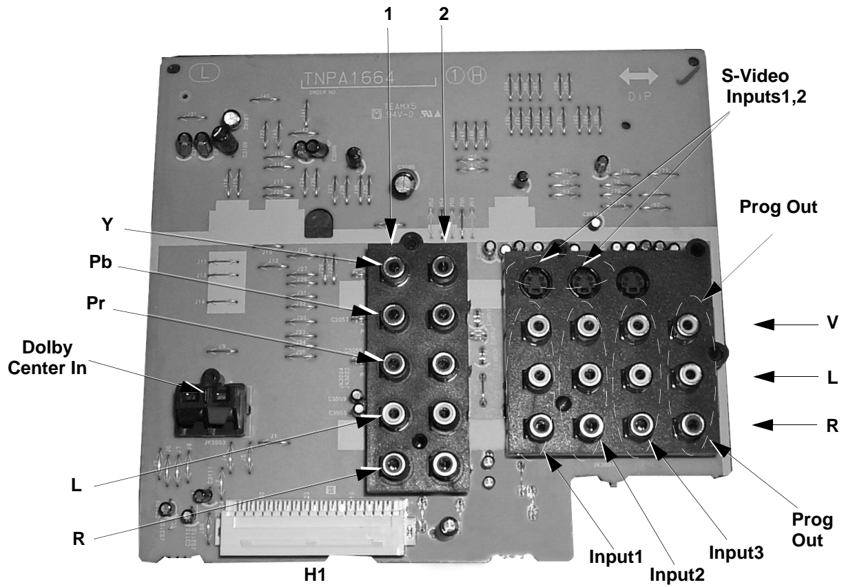
Figure 53. H-Board
