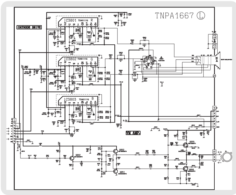
L-Board Voltage Measurements (IC & Transistors)
