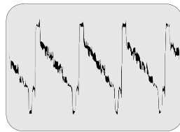
①⑦ A-Bboard IC001 Pin 30 - 1.86V p-p CVBS1
