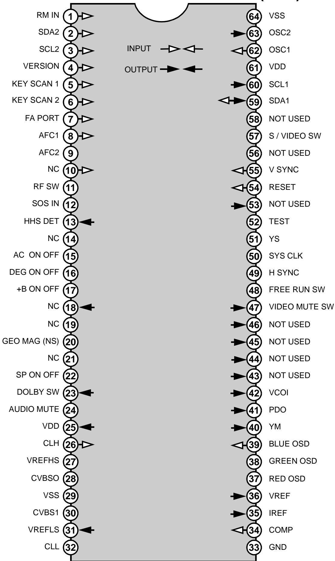
Figure 48. MPU IN/OUT Pins and Functions.
