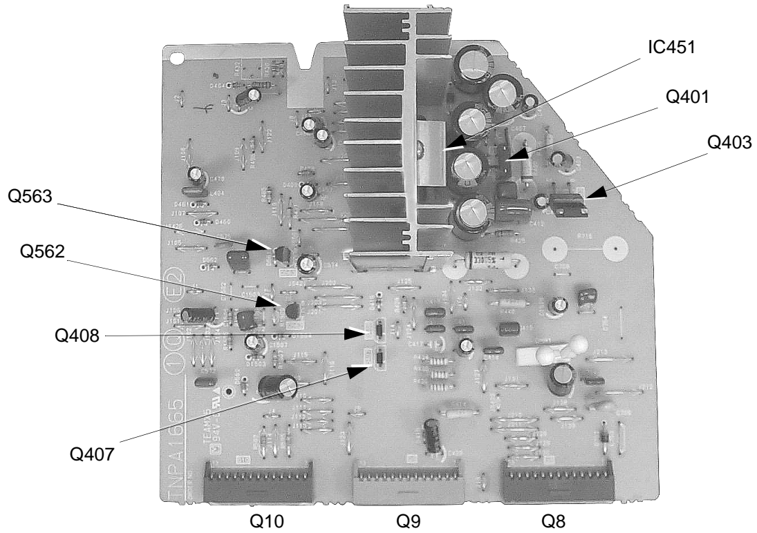
Figure 51. Q-Board
