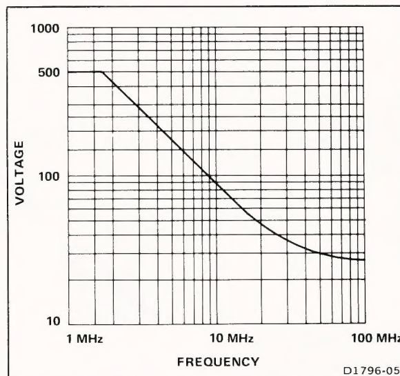
Fig. 3. Voltage vs. frequency derating.
