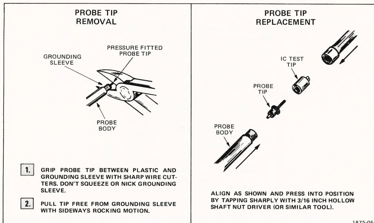
Fig. 4. Probe tip removal and replacement.
