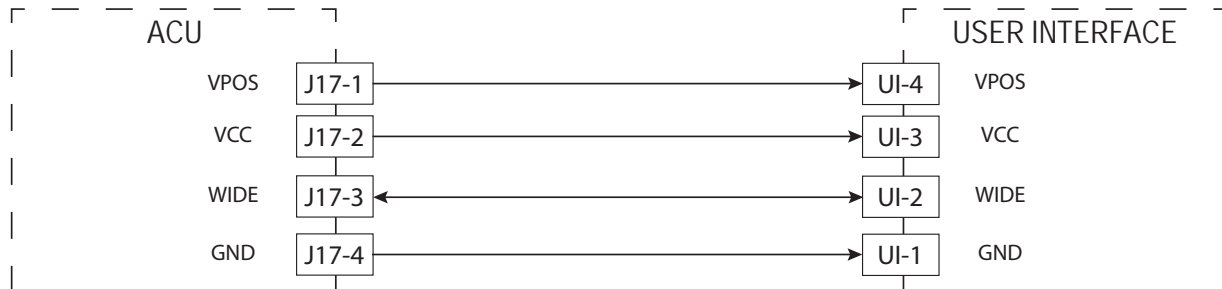
Figure 2 - User Interface Strip Circuit
