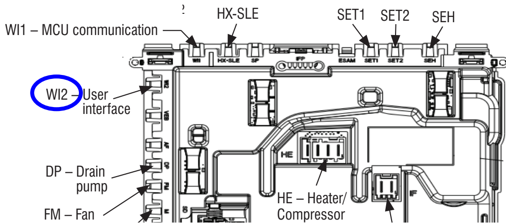
Figure 1 - User Interface Connector (W12)
