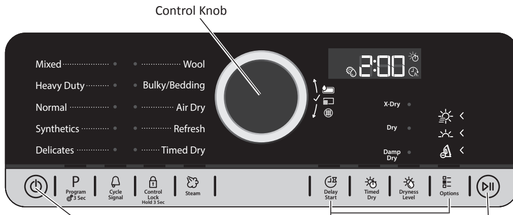
Figure 1- Service Diagnostic Mode/Test Cycle
