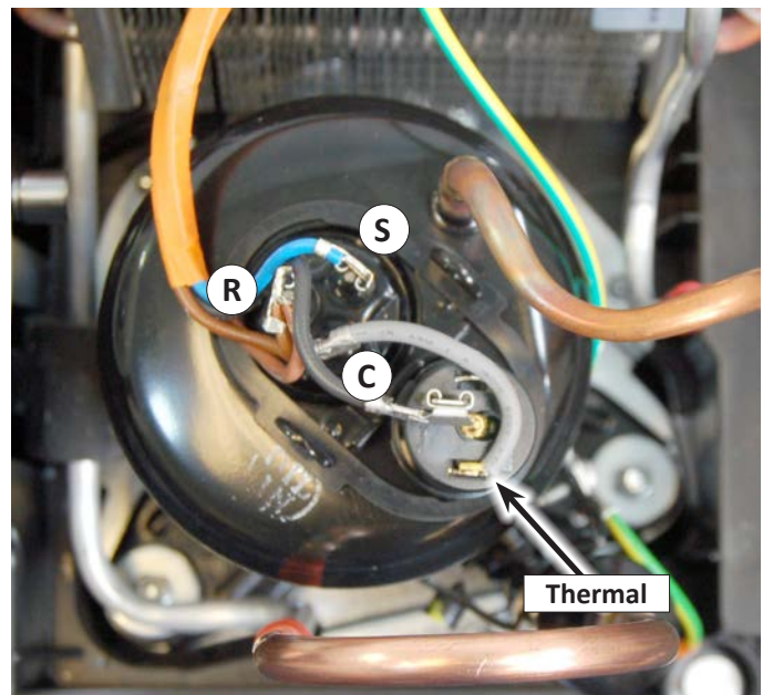
Figure 2 - Compressor Diagram
