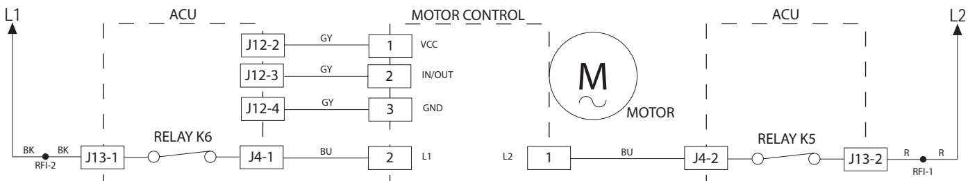
Figure 1 - Motor Strip Circuit
