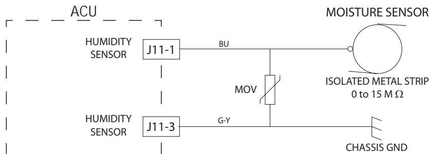
Figure 2 - Moisture Sensor Strip Circuit
