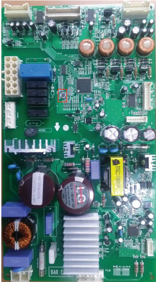
Main PCB
