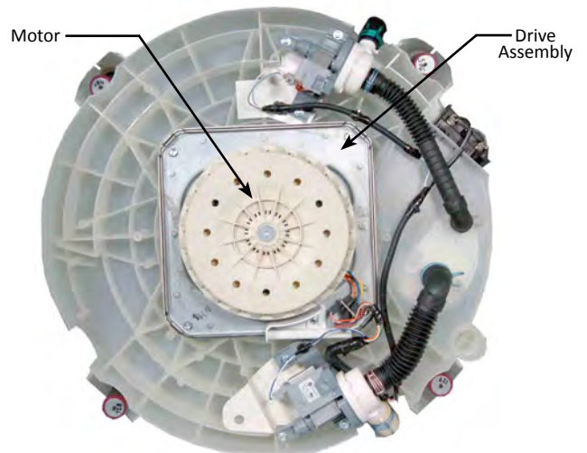
Figure 3 - Motor
