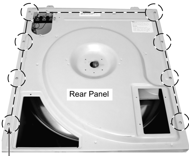
8 Rear Panel Screws
