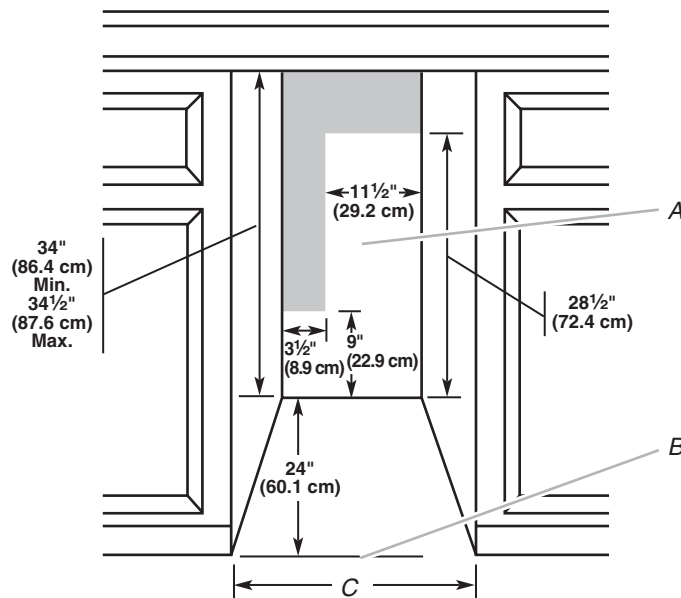
A. Recommended location for electrical and plumbing fixtures B. Floor level C. 15" or 18" (38.1 cm or 45.7 cm) depending on model
