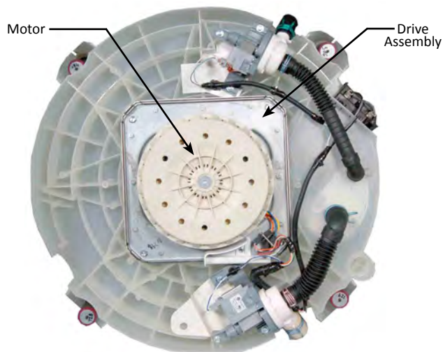
Figure 3 - Motor
