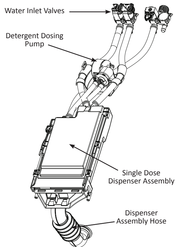
Figure 1 - Optimal Dispenser - Dosing Pump Location
