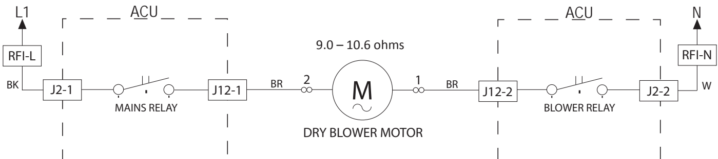
Figure 2 - Dry Blower Motor Strip Circuit
