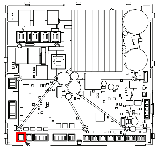
Figure 2 - Location of Baffle Solenoid Connector on ACU
