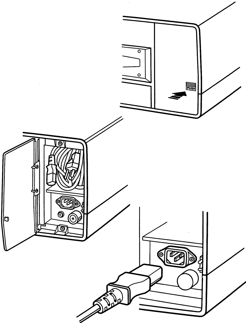
( Connector compartment )
