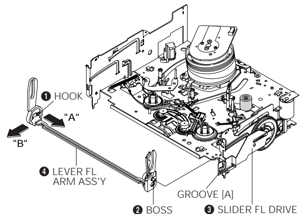
Fig. 4-7 Lever FL Arm Ass'y Removal
