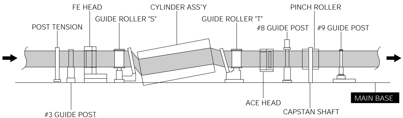
Fig. 4-4-2 Tape Travel Diagram
