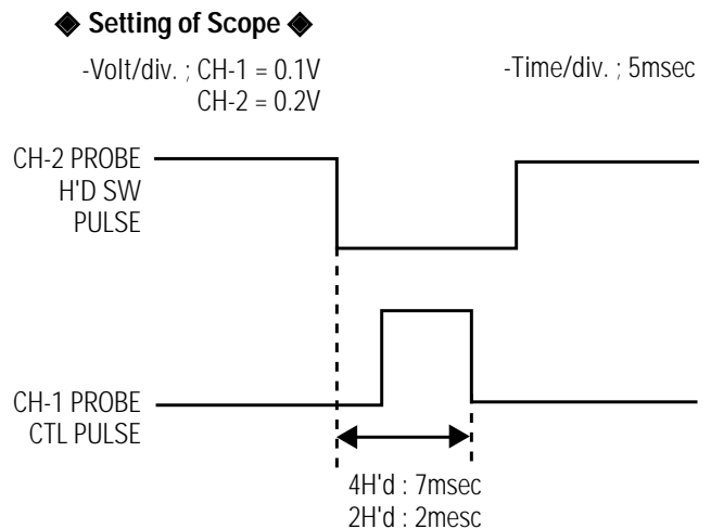
Fig. 4-5-4 Tracking Preset Adjustment
