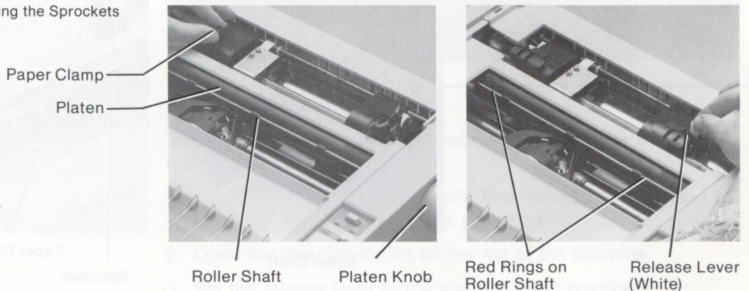
Figure 2-3. Adjusting the Sprockets
