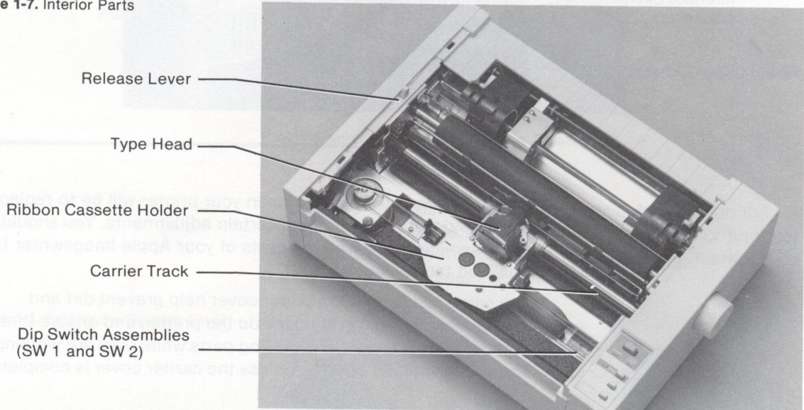
Figure 1-7. Interior Parts
